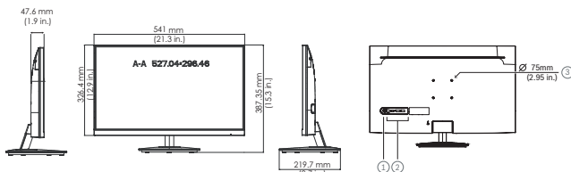
Dimensions High Performance LED monitor (24 in.)
